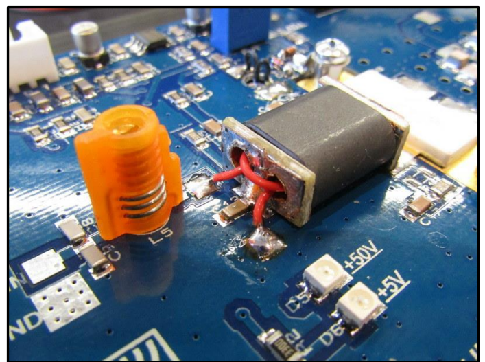
Figure 6d: Transformer winding detail.
