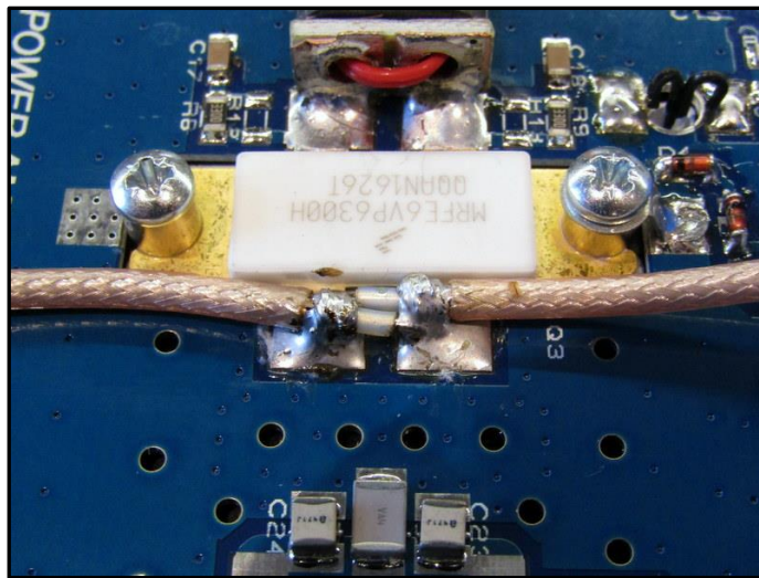
Figure 6: Transistor output coaxes.
