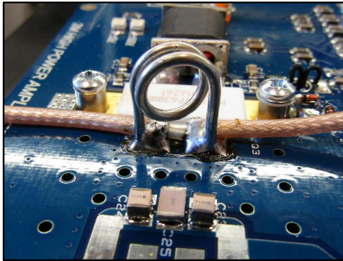
Figure 9: L4 mounting.
