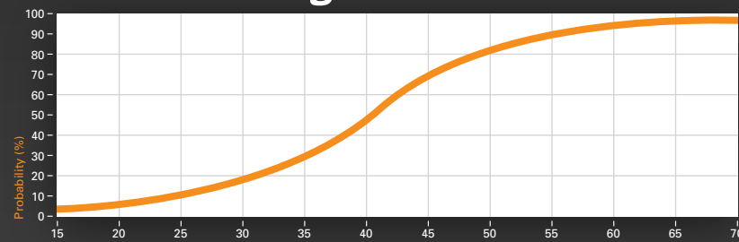
Incident Energy (cal/cm 2 ) Arc Thermal Performance Value (ATPV): Value is presented in calories per square centimeter represents the maximum capability for arc flash protection for a particular arc flash clothing.
