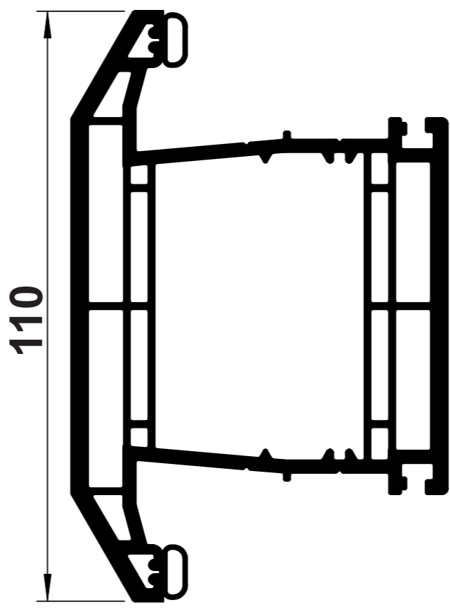
B14 BEVELLED 'T' MIDRAIL
