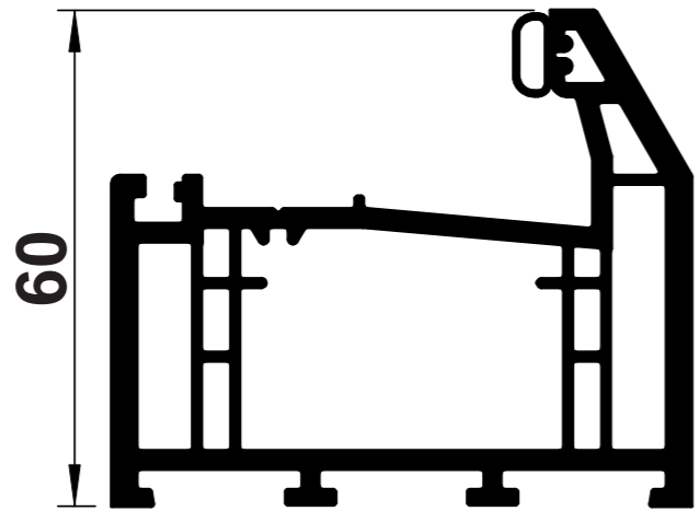
B02 BEVELLED INTERMEDIATE OUTER FRAME
