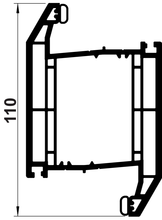
B15 BEVELLED 'Z' MIDRAIL
