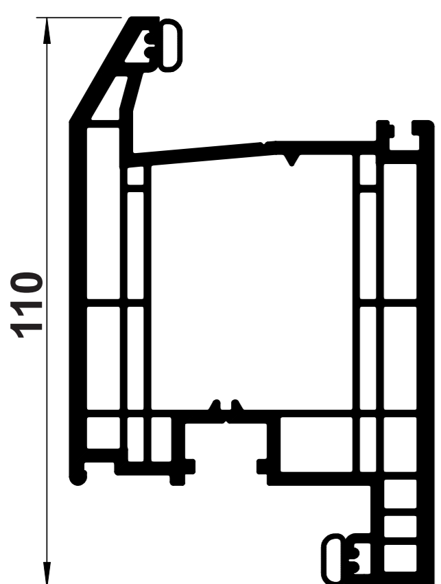
B40 BEVELLED 'Z' DOOR SASH
