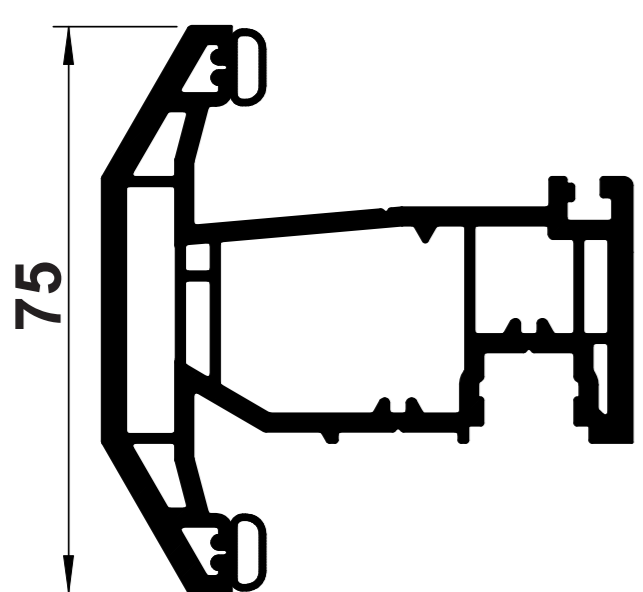
B30 BEVELLED 'T' CASEMENT SASH
