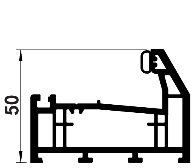
B01 BEVELLED SLIM OUTER FRAME
