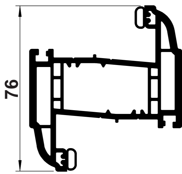
B23 OVOLO INTERMEDIATE 'Z' TRANSOM
