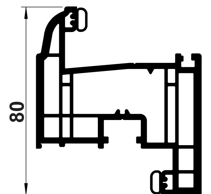
B38 OVOLO 'Z' TILT & TURN SASH
