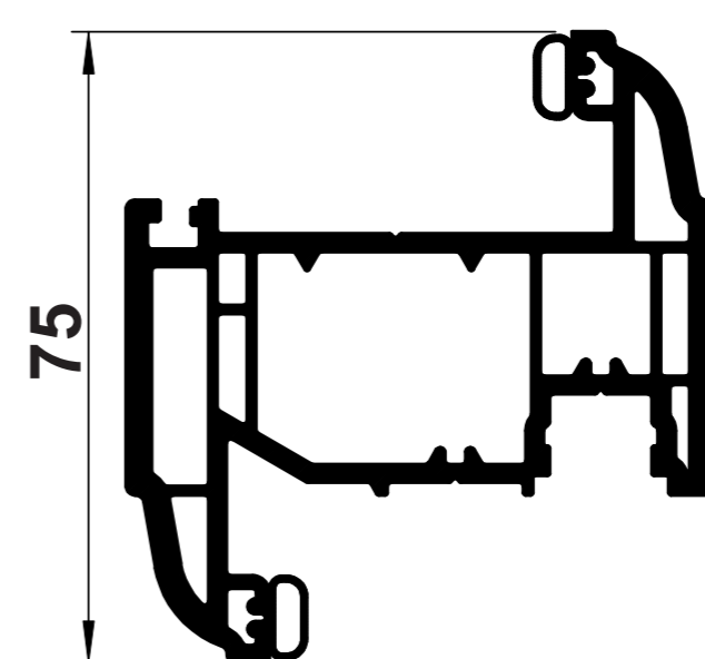
B36 OVOLO 'Z' CASEMENT SASH
