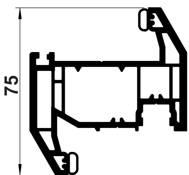
B31 BEVELLED 'Z' CASEMENT SASH
