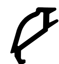
B60 28mm OVOLO GLAZING BEAD
