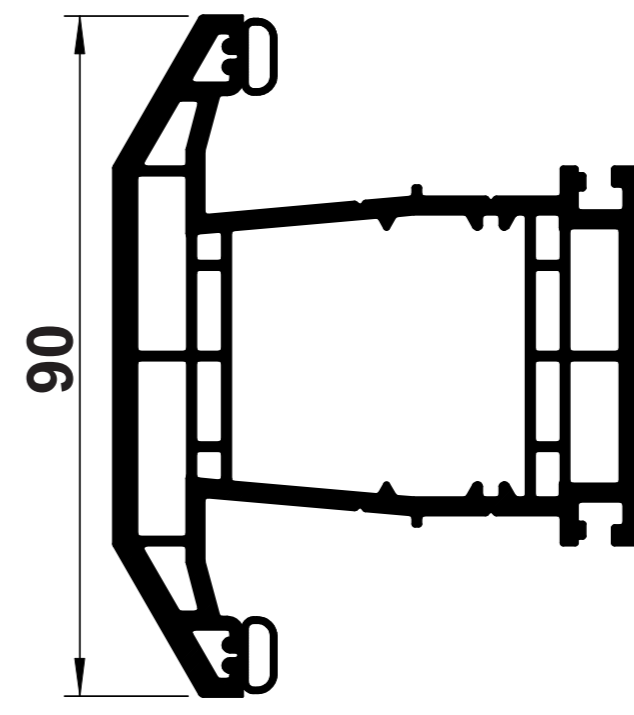
B16 BEVELLED LARGE 'T' TRANSOM
