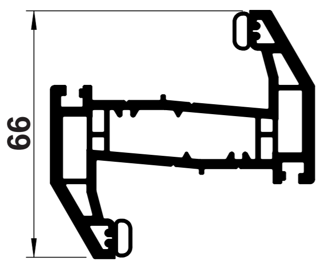
B11 BEVELLED SLIM 'Z' TRANSOM
