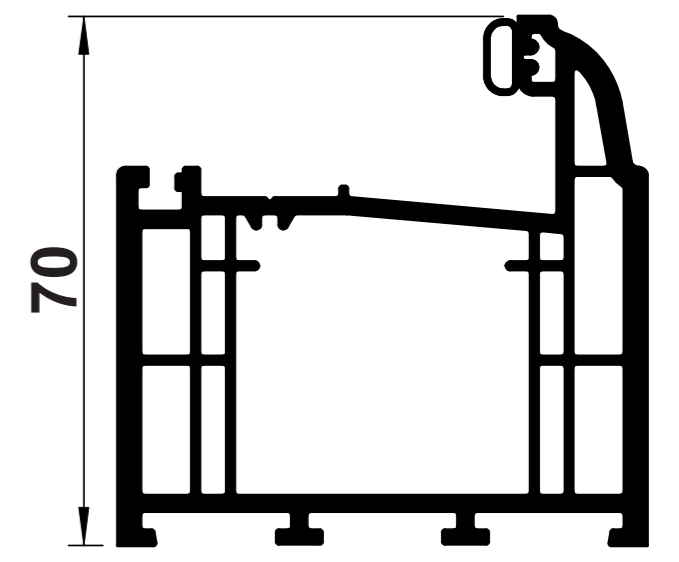
B07 OVOLO LARGE OUTER FRAME
