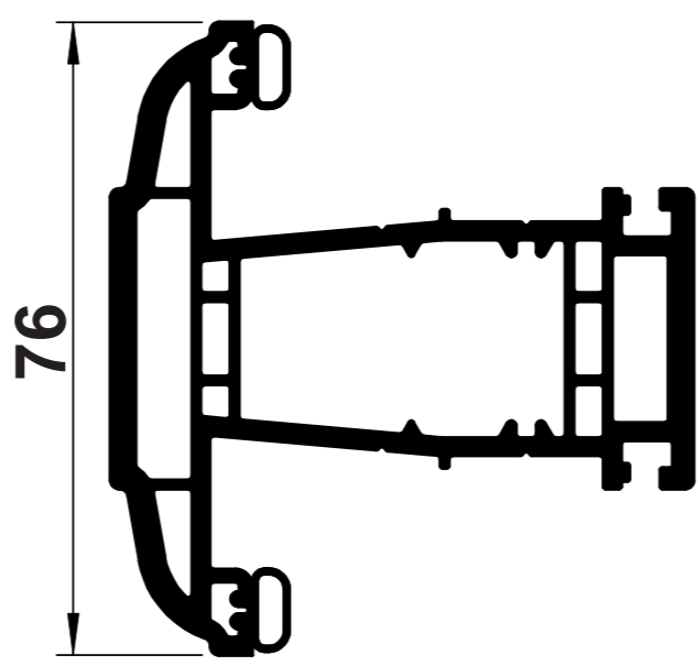
B22 OVOLO INTERMEDIATE 'T' TRANSOM
