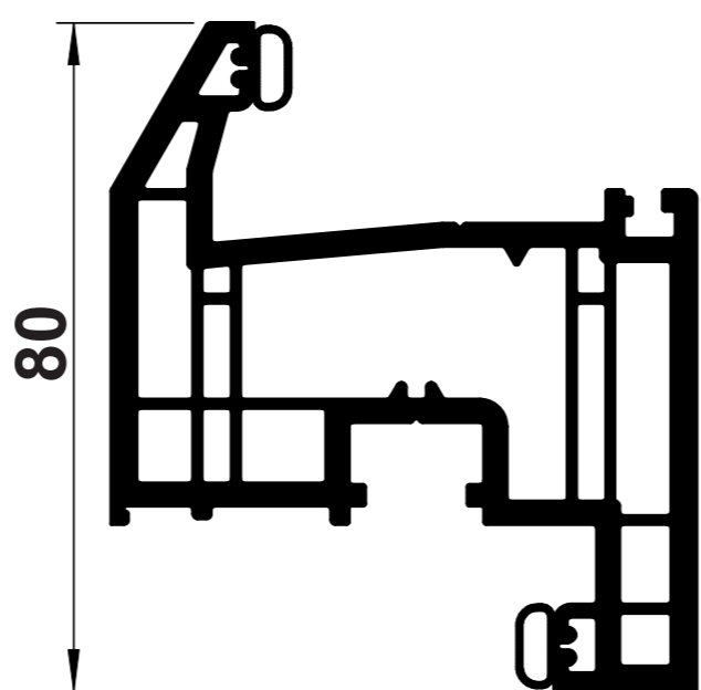
B33 BEVELLED 'Z' TILT & TURN SASH
