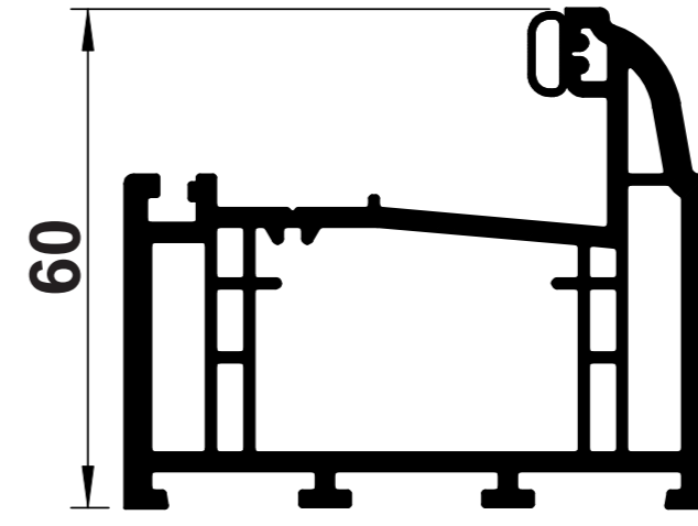
B06 OVOLO INTERMEDIATE OUTER FRAME
