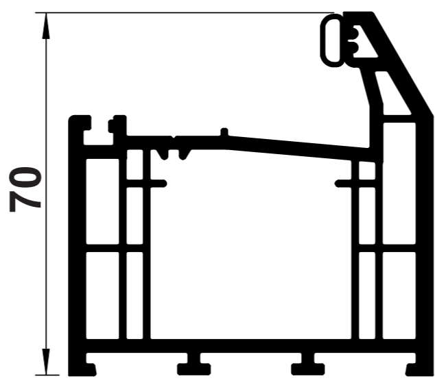
B03 BEVELLED LARGE OUTER FRAME
