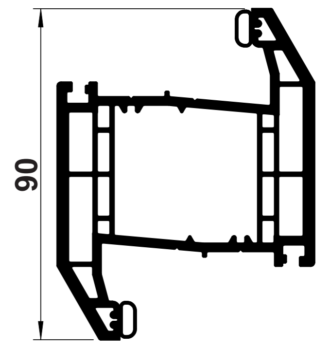
B17 BEVELLED LARGE 'Z' TRANSOM
