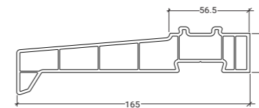
LCL165 165mm Cill
