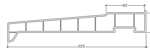
LSL225 225mm Cill
