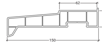
LSL150 150mm Cill
