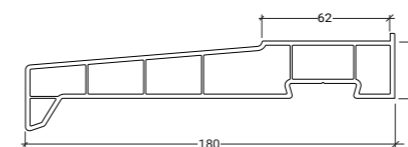
LSL180 180mm Cill
