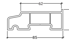
LSL085 85mm Stub Cill
