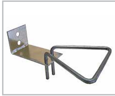
P-312 / P-316 DOUBLE ADJUSTABLE ANCHOR (2)
