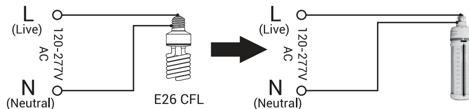
E26 LED Lamp
