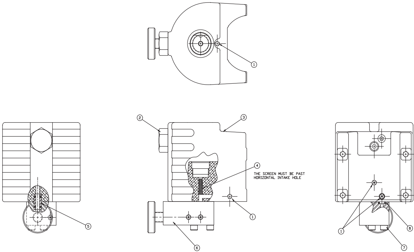
Figure 2 - 42415SR Pump Body Assembly
