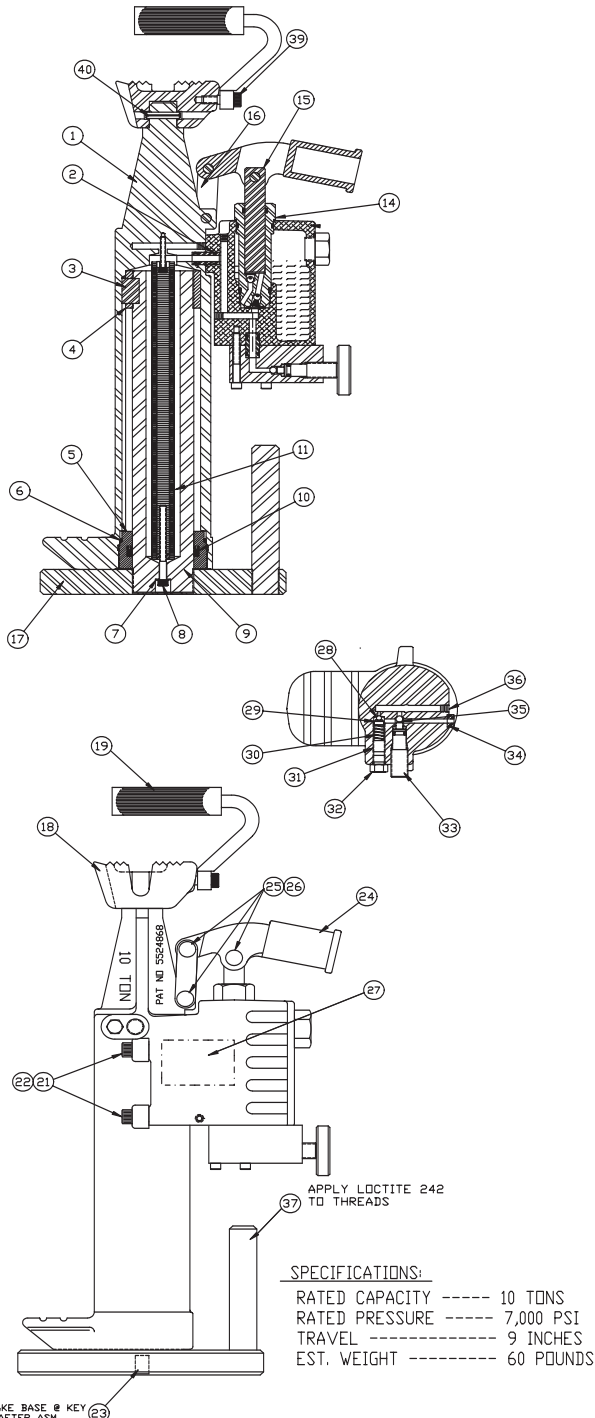
Figure 1 - Main Assembly
