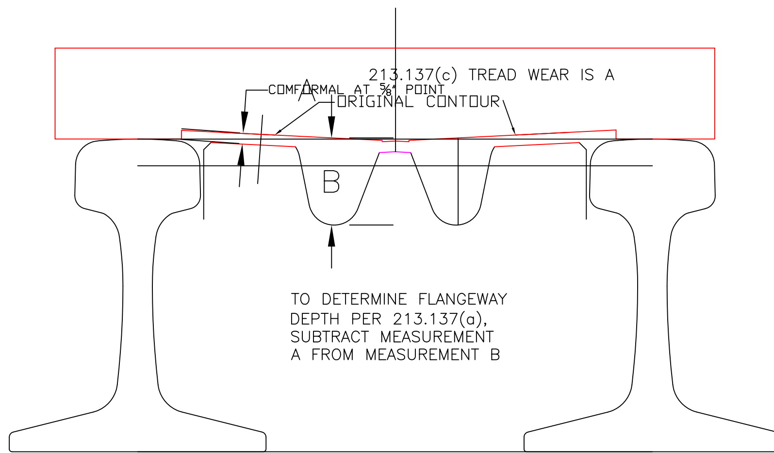
CONFORMAL GAGE FOR CHECKING TREAD WEAR AND FLANGEWAY DEPTH AT POINT
