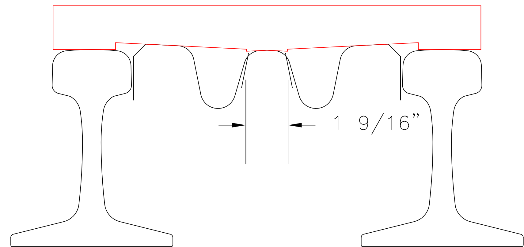
CONFORMAL GAGE FOR CHECKING TREAD WEAR AND FLANGEWAY DEPTH AT 1 9/16" SPREAD
