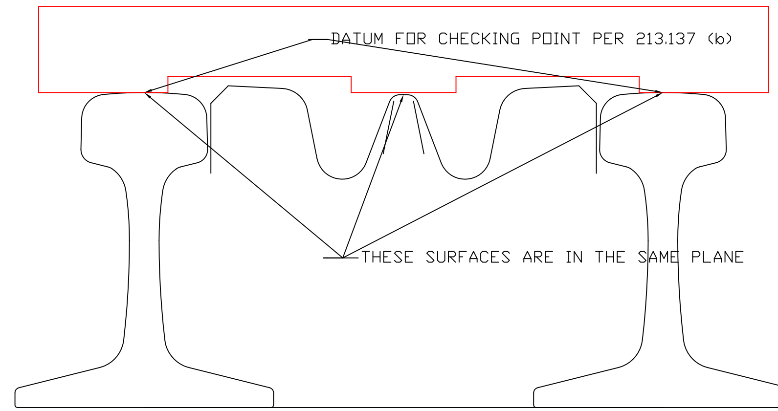
GAGE TO CHECK 5/8" POINT WEAR ON CONFORMAL FROGS
