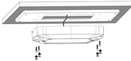
Surface Mount with Adapter Plate* (*available as an optional accessory)
