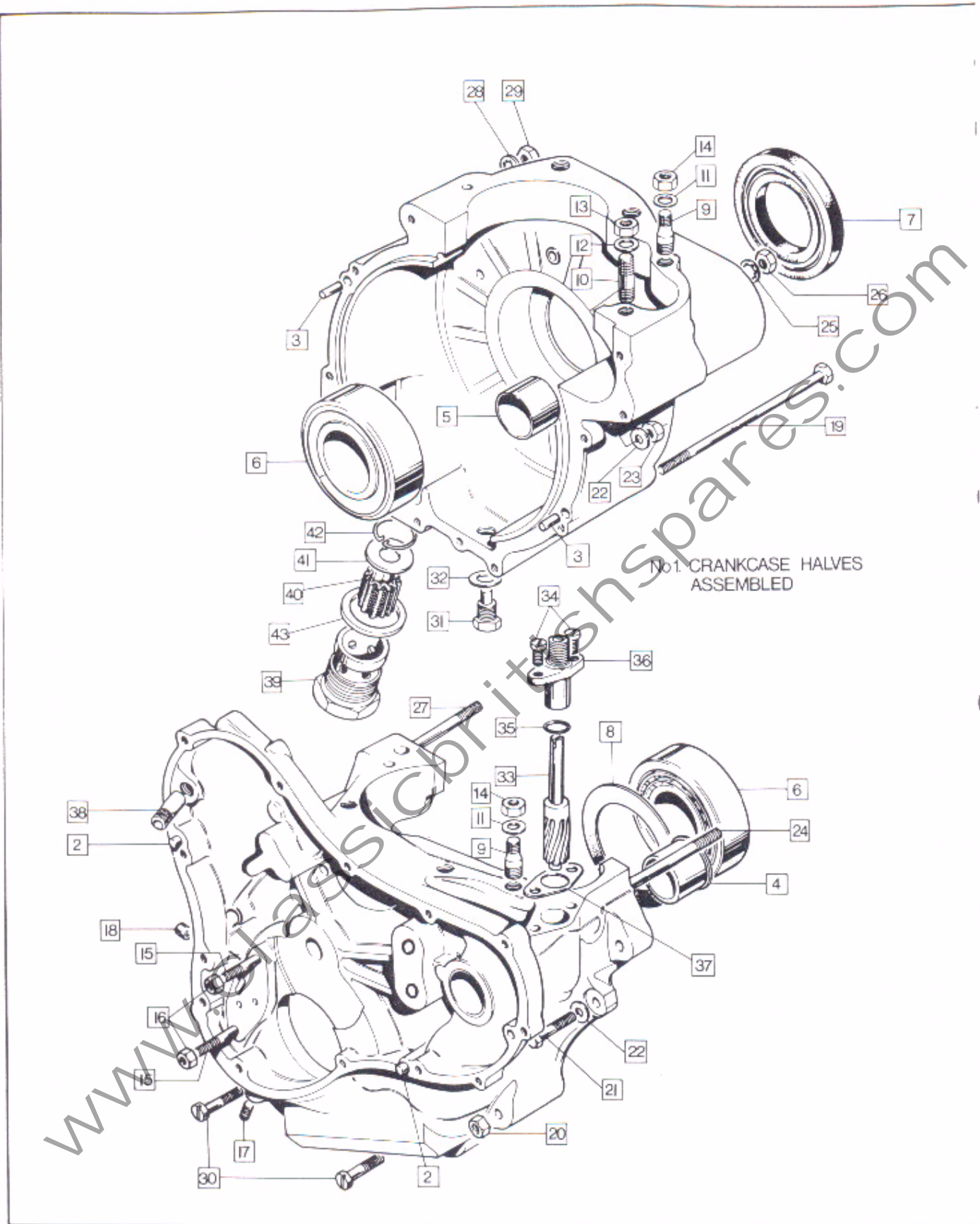
850 Engine: Crankcases, Filter, Breather, Tachometer Drive
