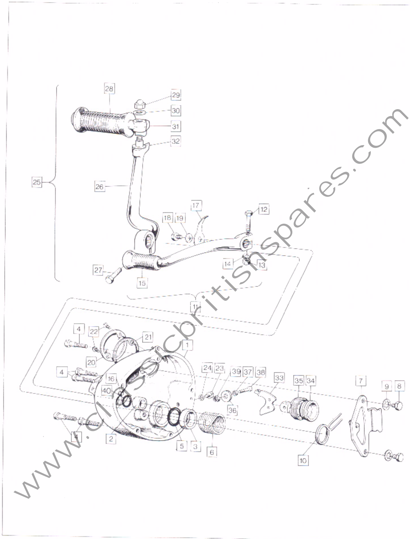
Gearbox: Outer Cover
