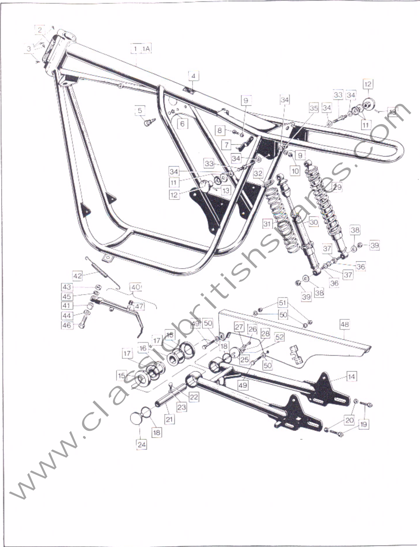
Frame, Swinging Arm, Suspension Units
