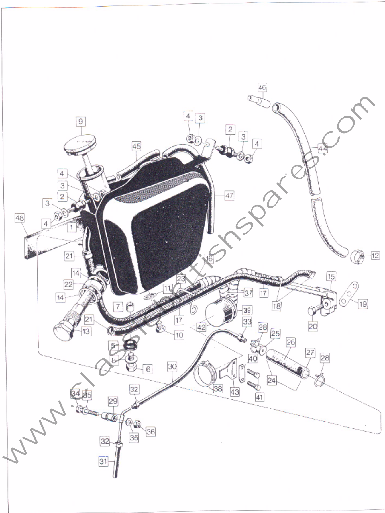
Oil Tank, Oil Pipes, Junction Block, Rear Chain Oiler and Full Flow Oil Filter
