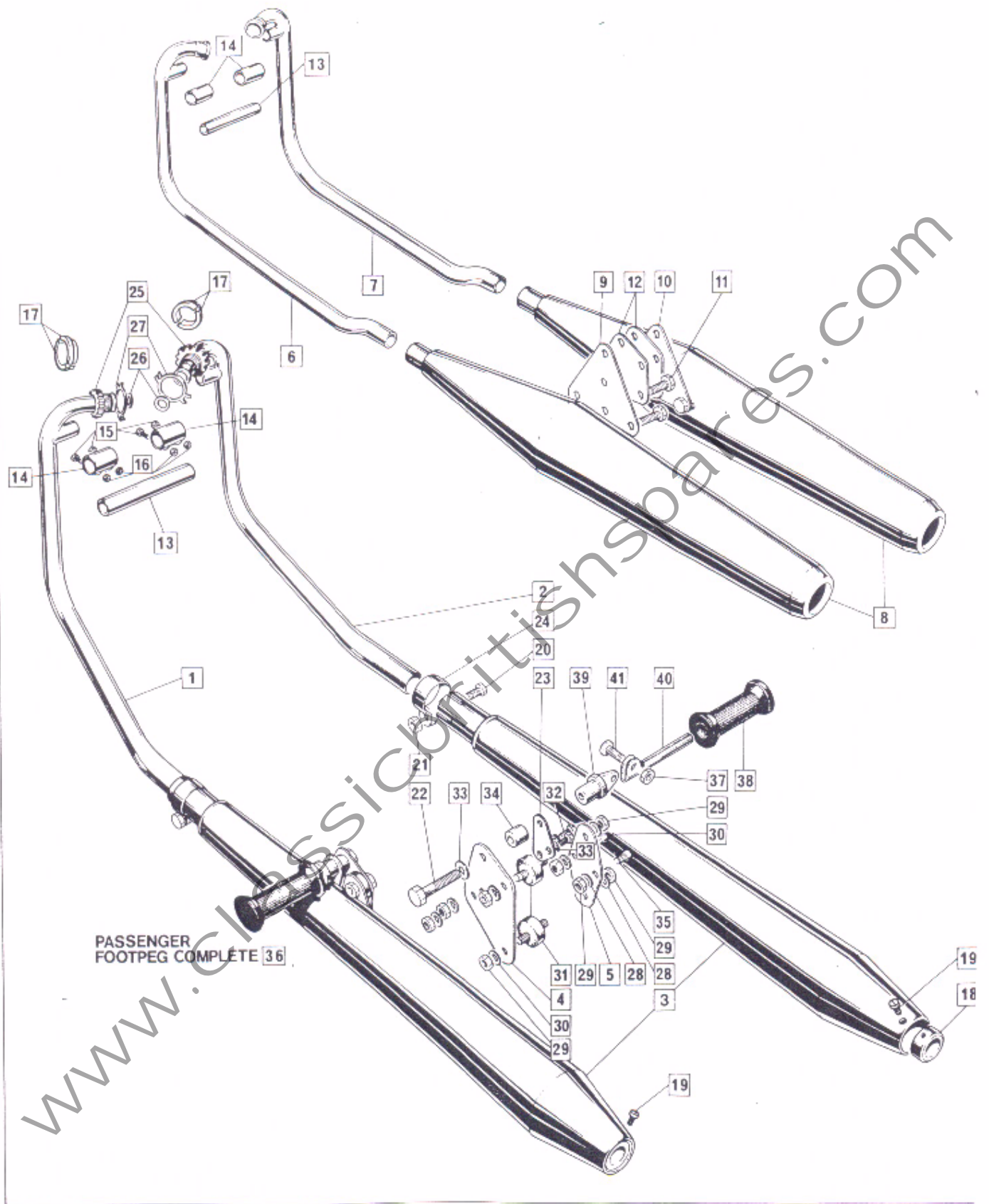
850 Exhausts, Mufflers, Mutes, Passenger Footpegs
