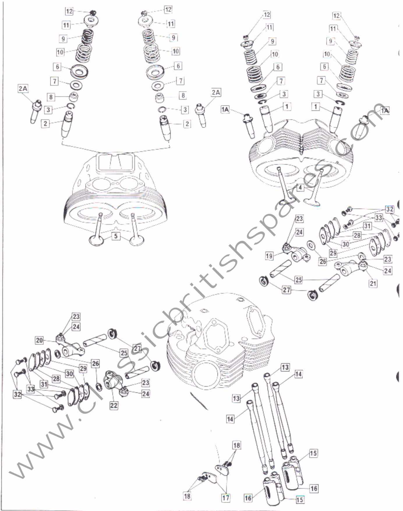
Valve Gear
