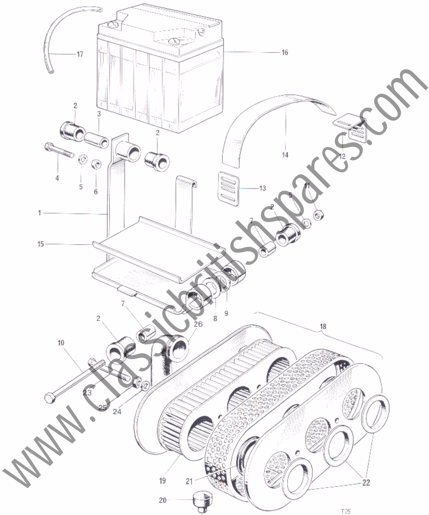
Fig. 27. BATTERY CARRIER AND AIR FILTER
