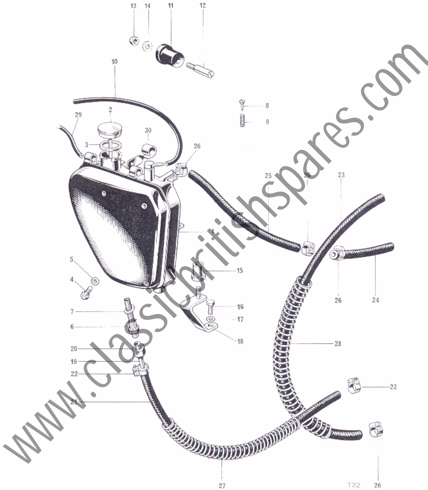
Fig. 26. OIL TANK
