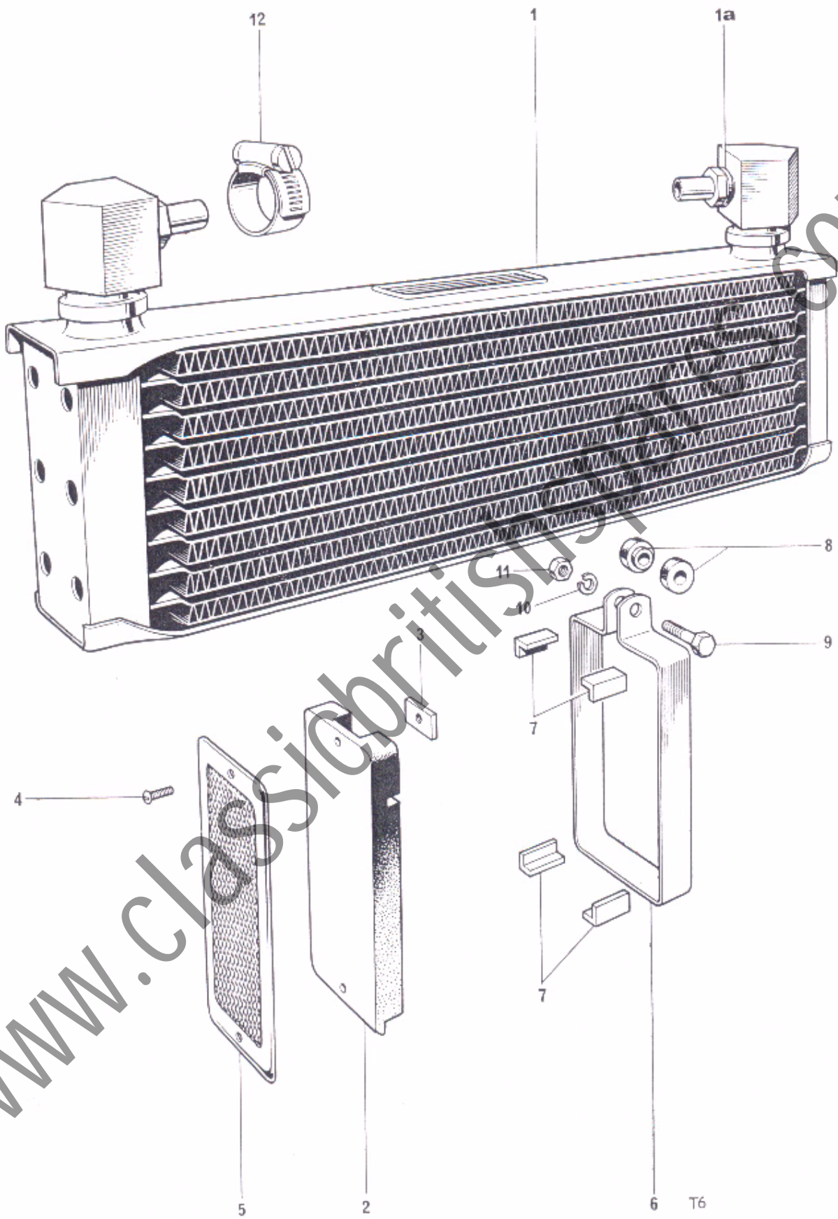
Fig. 24. OIL COOLER
