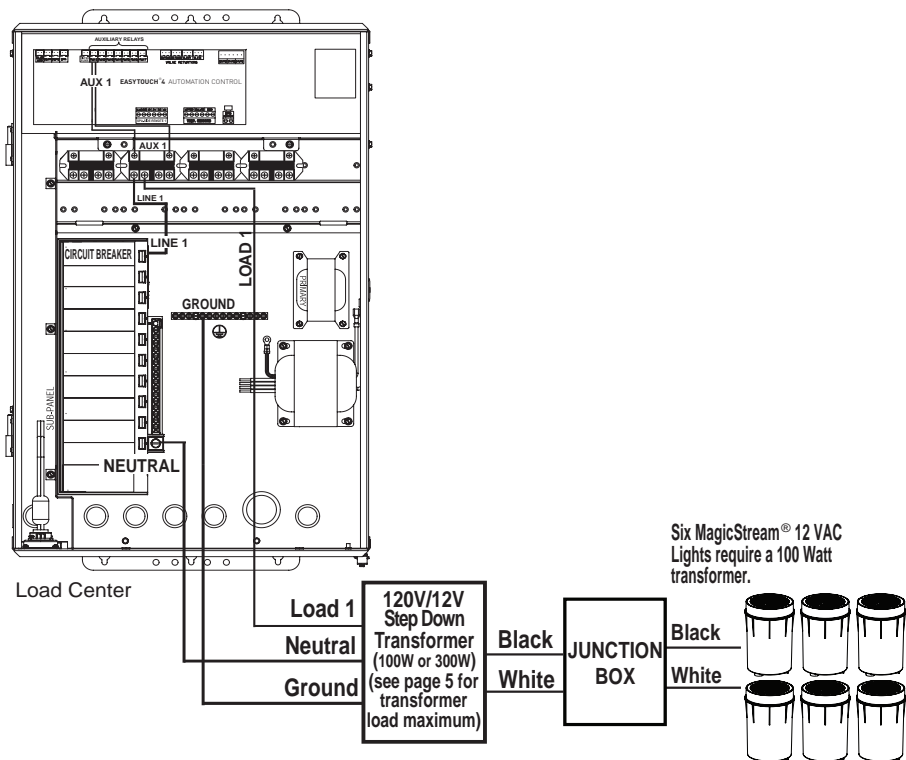
MagicStream® Laminar to EasyTouch or IntelliTouch Control System Load Center Wiring Connection Diagram
