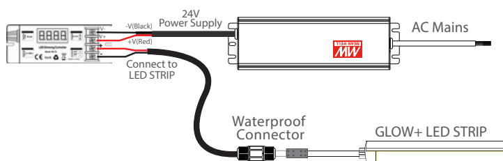
With Dimmer wiring diagram
