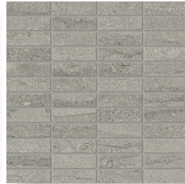
Fossil
