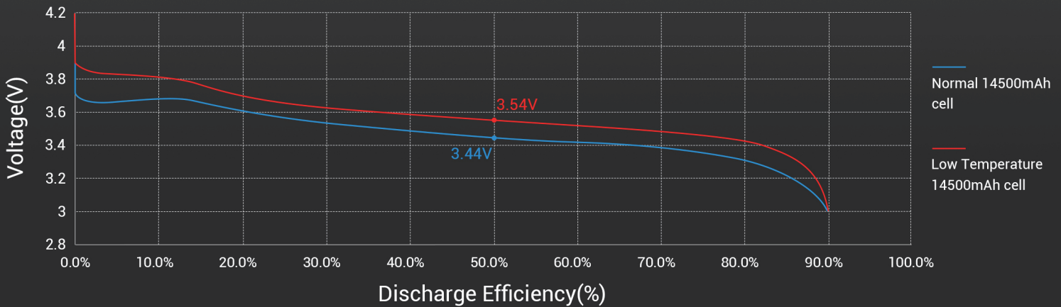
157W Discharge Curve@ -10^{\circ}\text{C}
