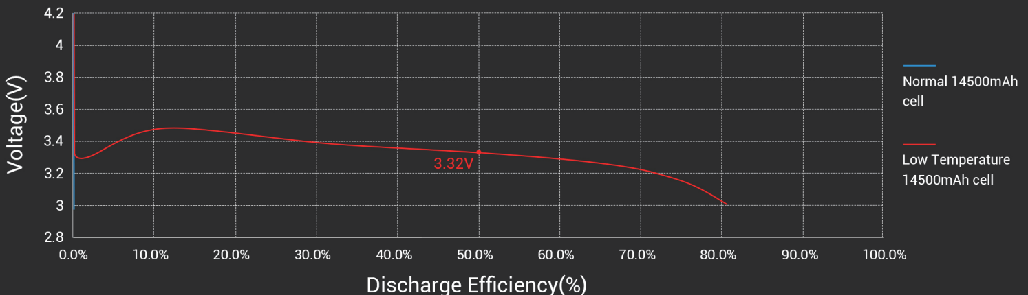
157W Discharge Curve@ -30^{\circ}\text{C}
