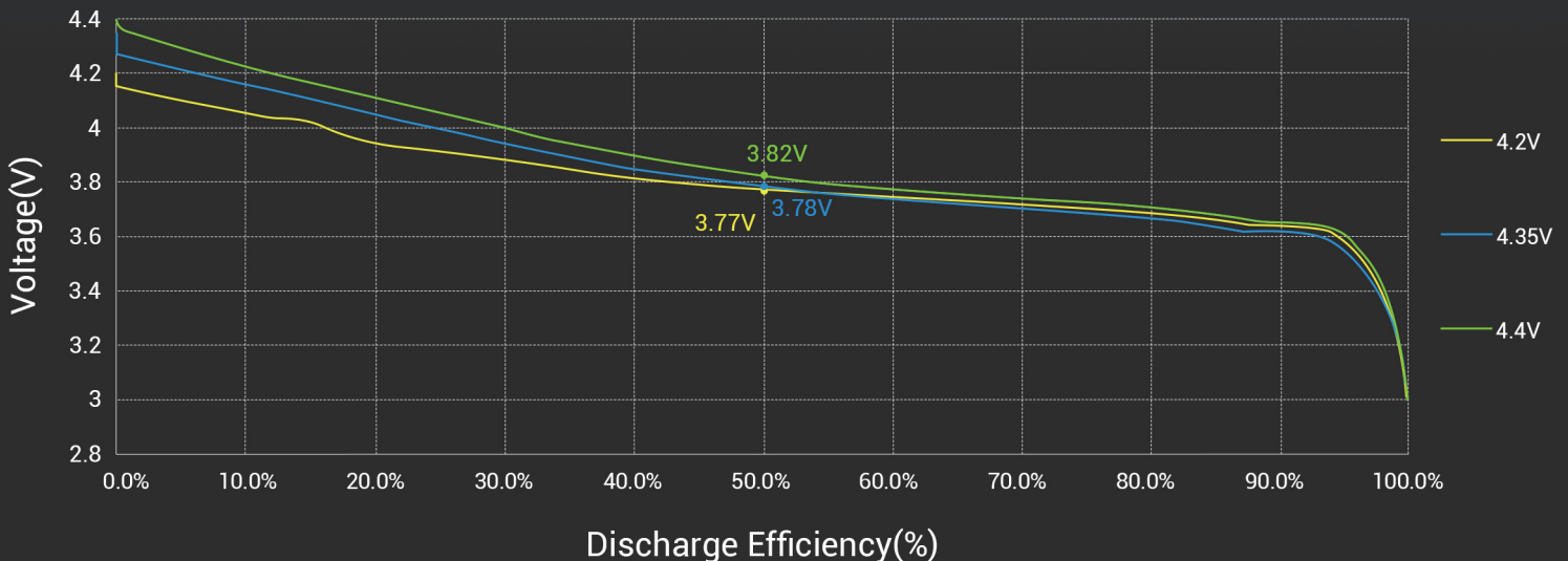
Discharge Curve @ 0.5C
