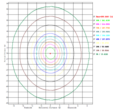
120° (Optional)
