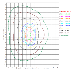
Type IV
