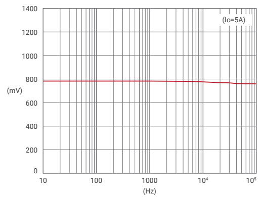
Frequency Characteristic
