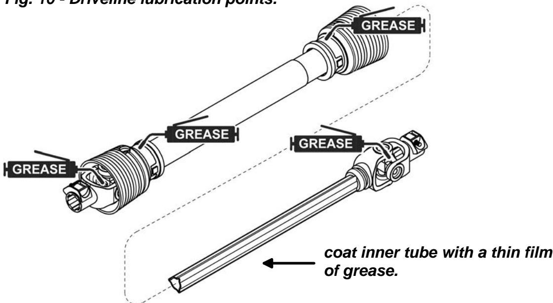
Fig. 10 - Driveline lubrication points.
