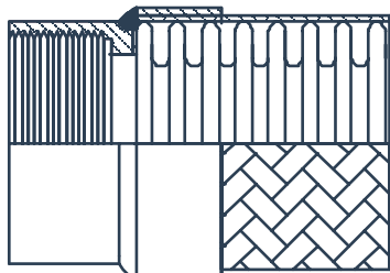
Half Coupling
