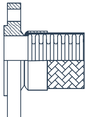
Slip-On Raised Face 150, 300,600 lb Drilling
