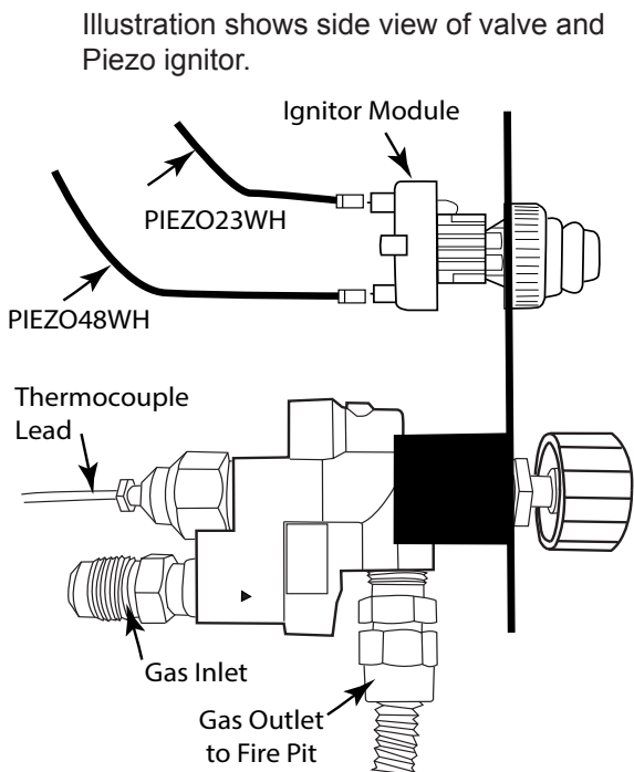
Fig. 4 TMSI typical installation.
