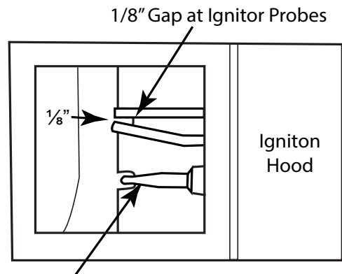
Thermocouple Fig. 5 Proper alignment of probes and thermocouple.
