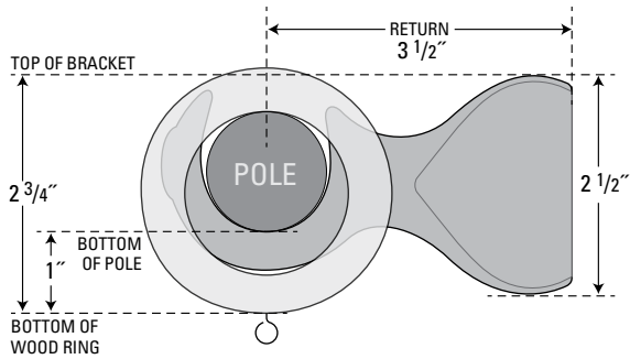
1 3/8" European Bracket - 13-223
