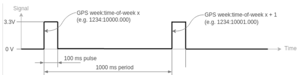
Figure 5.5.: An illustration of time pulse function
