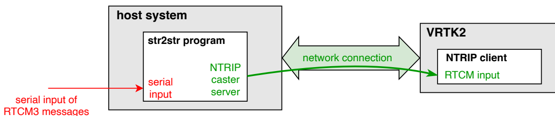
Figure 5.15.: Workflow diagram of the str2str program combined with the Vision-RTK 2
