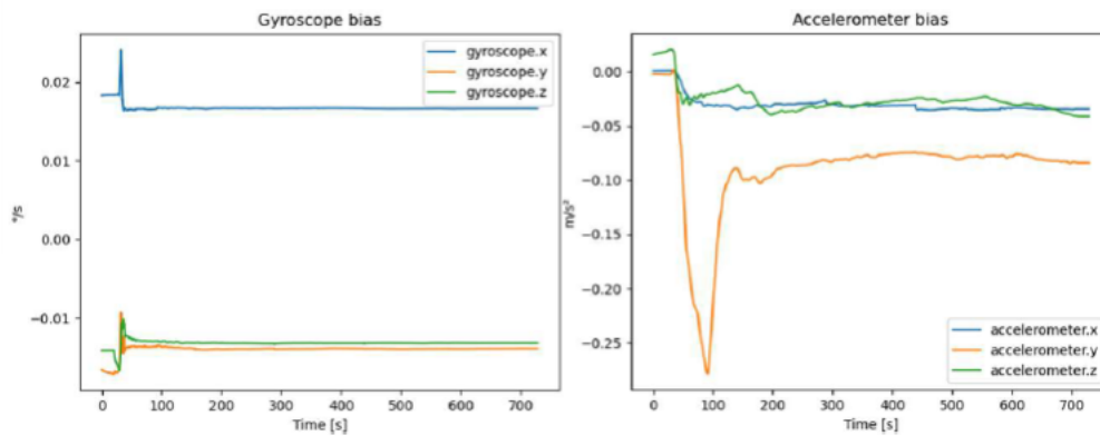
Figure 5.26.: Gyroscope and accelerometer biases over time
