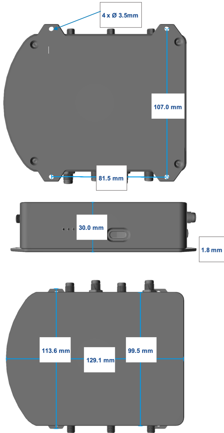
Figure 3.7.: Dimensions of the Vision-RTK 2's enclosure
