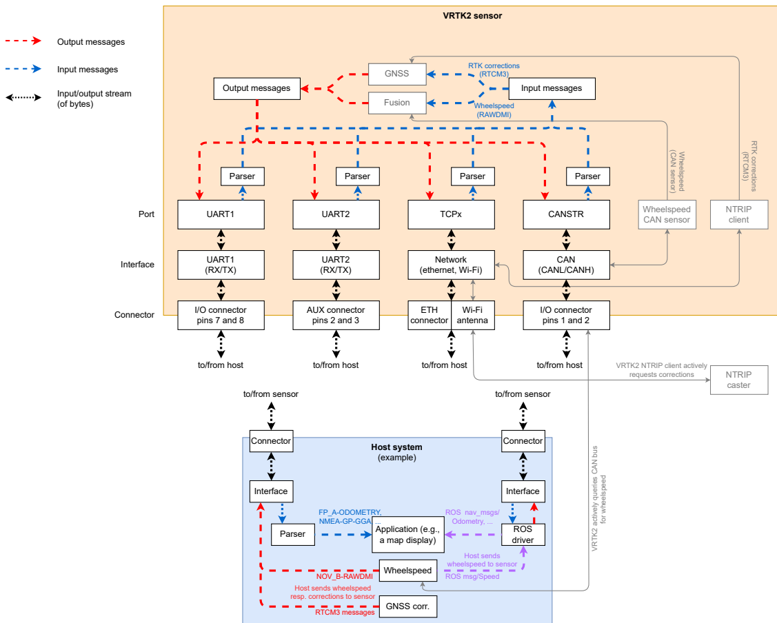
Figure 5.6.: Input/output system overview
