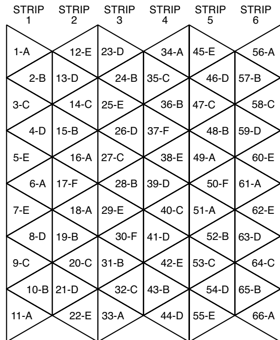
ASSEMBLY DIAGRAM
