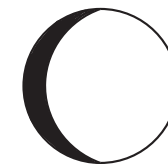
Waxing Gibbous
