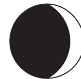
Waxing Crescent
