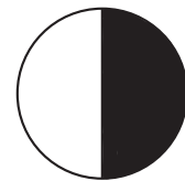
Third Quarter
