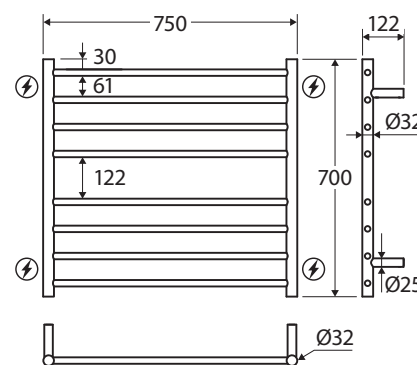
⚡ Wiring Positions
