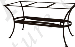
LARGE DINING TABLE BASE D: 26.5" W: 53.5" H: 28"
