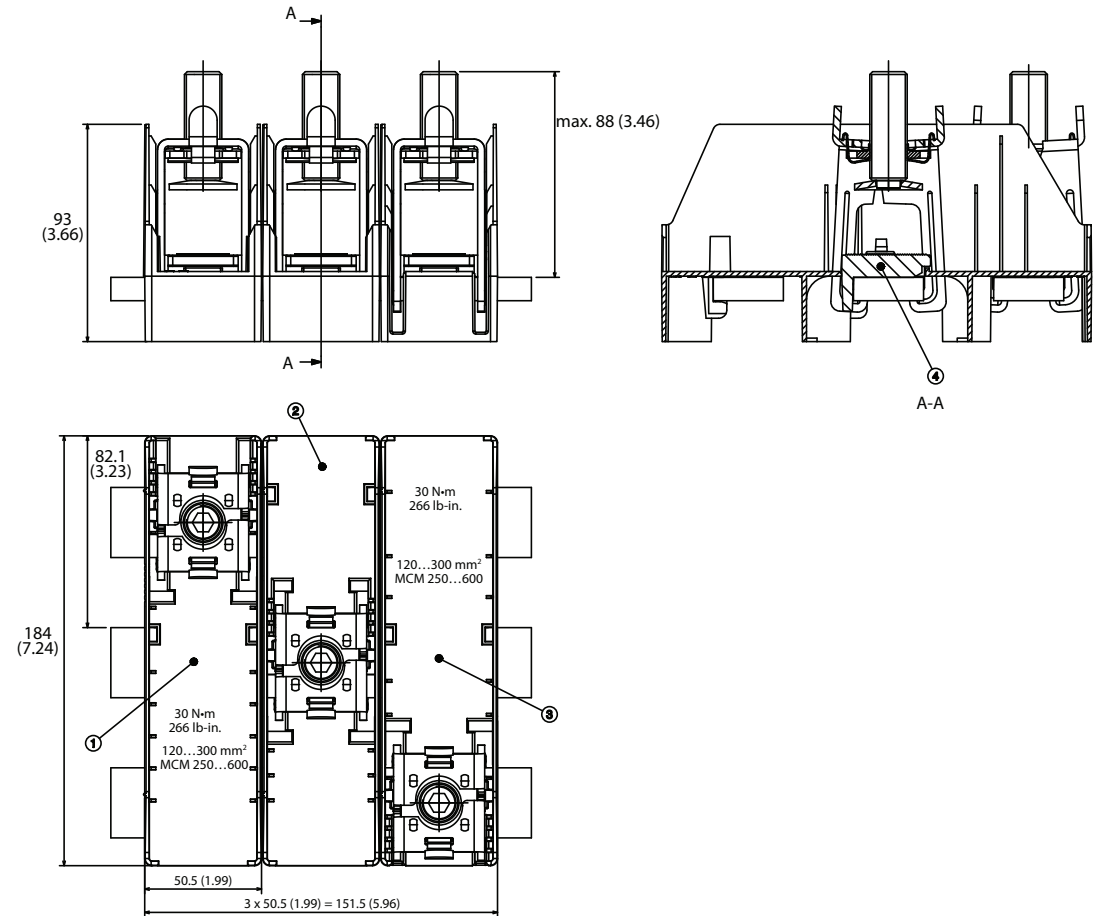
Figure 45 - Cat. Nos. 141A-VU3300R and -VU3300F
