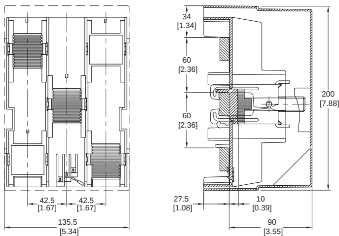
Figure 44 - Cat. Nos. 141A-VN3185, -VN3300R, and -VN3300F
