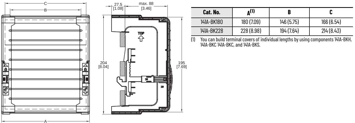
Figure 49 - 141A-BK180, -BK228 Terminal Covers
