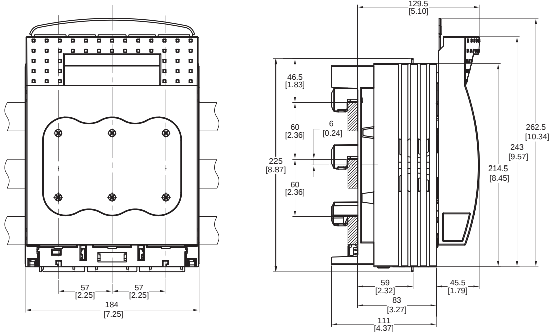
Figure 32 - Cat. No. 141A-NFJ400
