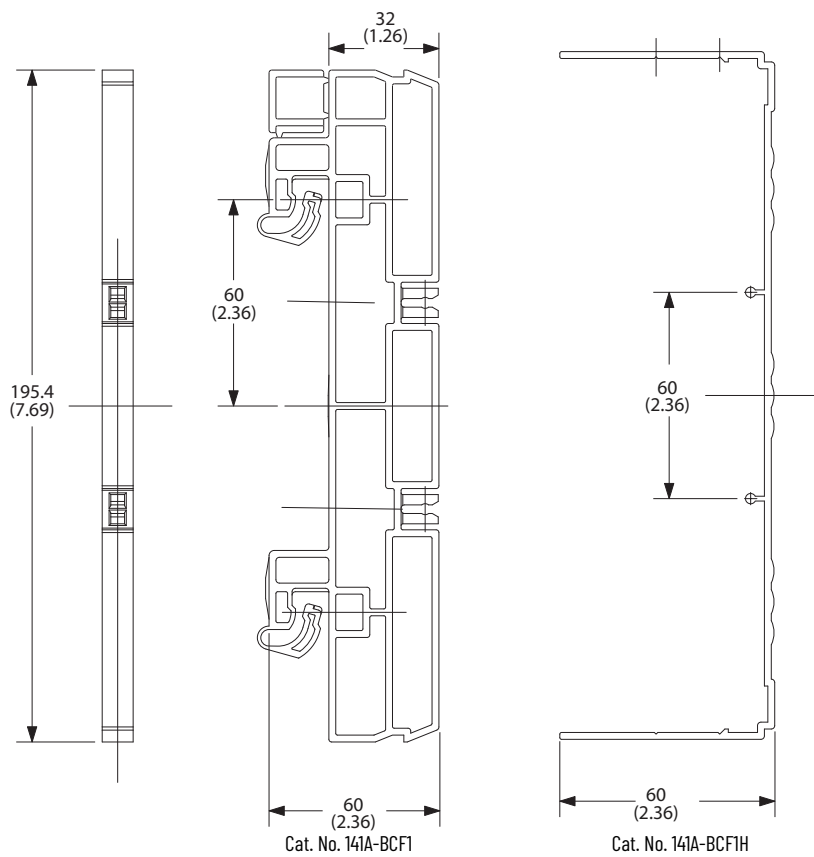
Figure 50 - Cat. Nos. 141A-BCF1, 141A-BCF1H Busbar Cover and Cover Holder
