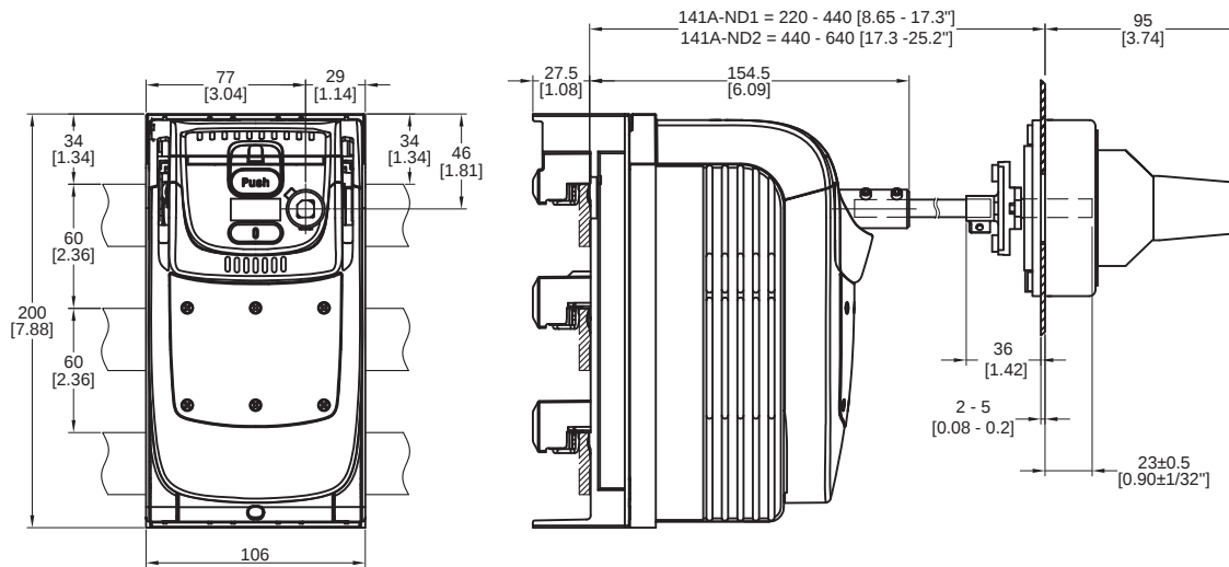
Figure 38 - 141A-N160SB Non-Fused Switch Disconnecter for External Rotary Operating Handle
