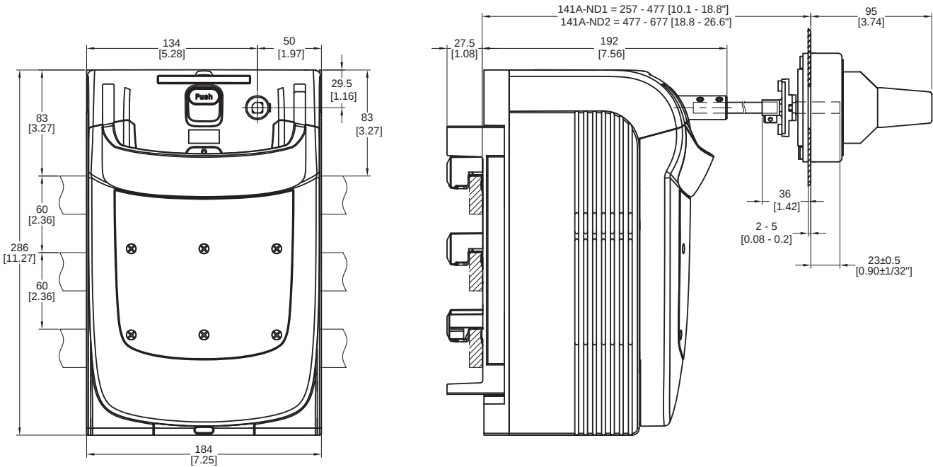
Figure 40 - 141A-NDN66 and 141A-NDRY66 Operating Handles
