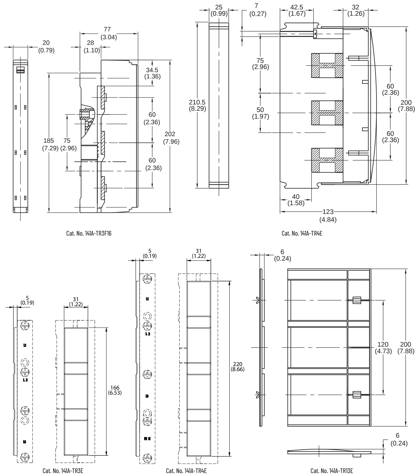
Figure 42 - Cat. Nos. 141A-TR3F16, -T13, -TR3E, -TR4E, and T13E Busbar Supports and End Covers
