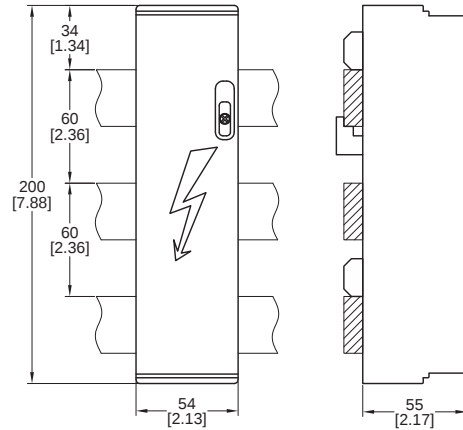
Figure 49 - 141A-BK180, -BK228 Terminal Covers
