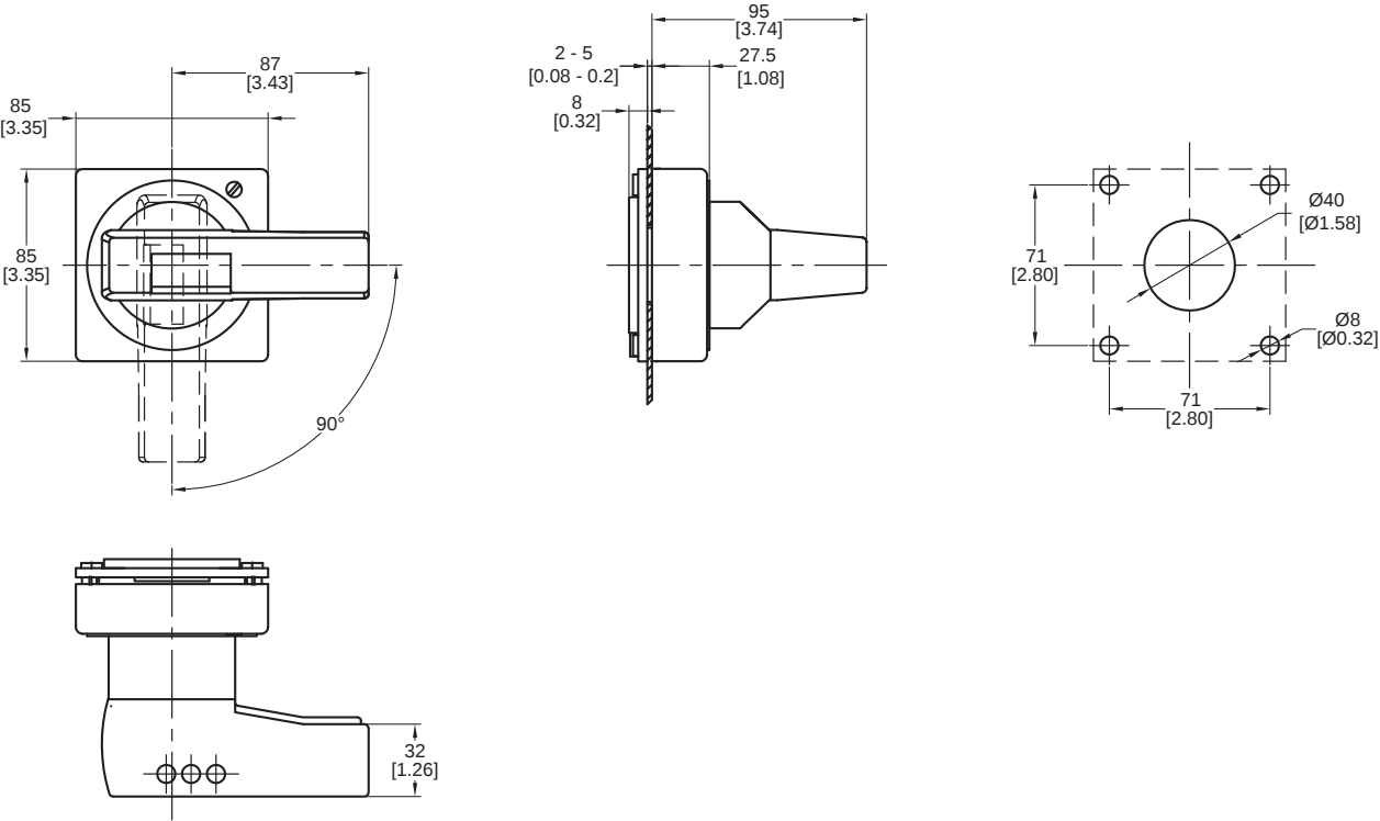
Figure 40 - 141A-NDN66 and 141A-NDRY66 Operating Handles
