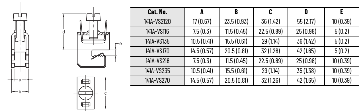
Figure 46 - 141A-VS... Terminals for Connecting to Busbars
