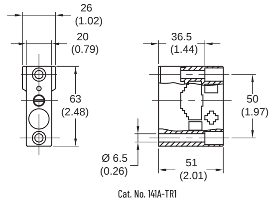
Cat. No. 141A-TR1
