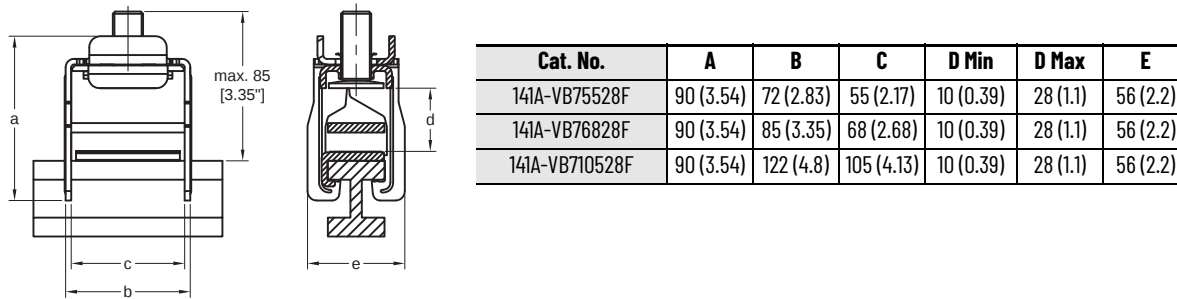
Figure 48 - 141A-BK1 Terminal Cover
