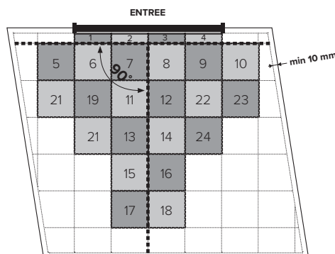
Fig. 2 Pose Fortelock INVISIBLE, BUSINESS
