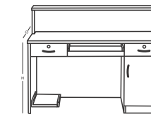
Reception Table FNS - Rec11a 1500W x 600D x 1100H FNS - Rec11b 1800W x 600D x 1100H
