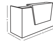
Reception Table FNS - Rec10a 1800W x 600D x 1100H FNS - Rec10b 2400W x 600D x 1100H
