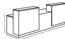
Reception Table FNS - Rec07a 2400W x 750D x 1100H FNS - Rec07b 3000W x 750D x 1100H
