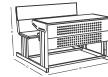
FNS - SD-90-42750 DESK 1066W x 930D x 750/450
