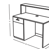
Reception Table FNS - Rec03a 1200W x 750D x 1100H FNS - Rec03b 1500W x 750H x 1100H
