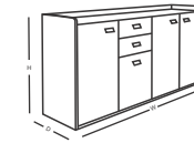
Storage Cabinet FNS - Cab29a 1800W x 450D x 750H
