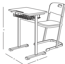
FNS-SD-35-6040750 CHAIR 420W x 525D x 820H DESK 600W x 400W x 760H
