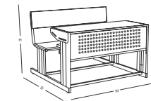
FNS - SD-96 DESK 1066W x 930D x 760/450
