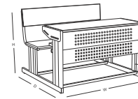
FNS - SD-PWD-760 DESK 1066W x 830D x 730/452
