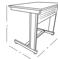
FNS-SD-37-604076 DESK 900W x 600D x 750H
