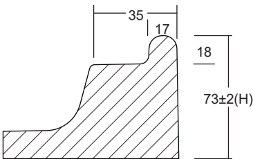
PRODUCT DIMENSIONS EDGE PROFILE
