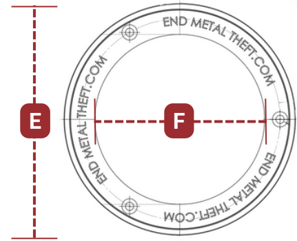
Escutcheon Front View
