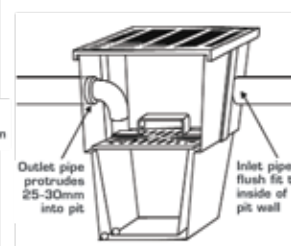
DIAGRAM C INSTALLATION
