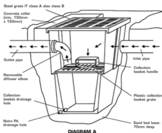
DIAGRAM A
