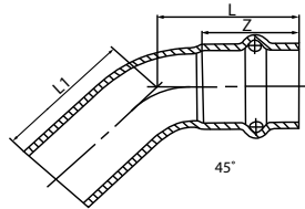
45° ELBOW M + F
