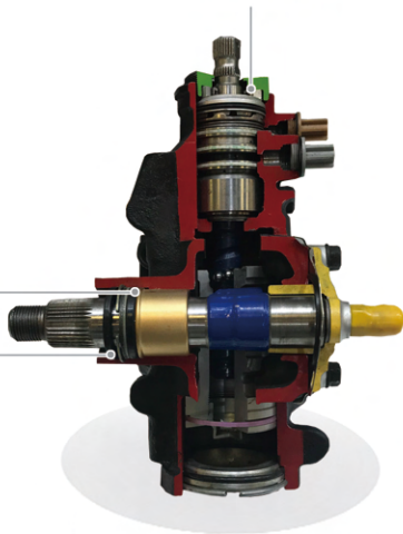
Input Seal
