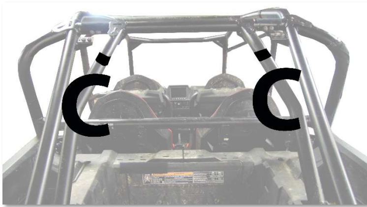
Figure 3: Tabs on the top cap will wrap around the roll bar.
