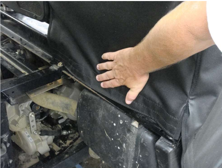
Figure 8.1 - square rear of enclosure to cab and attach rear enclosure Velcro tabs to installed Velcro strips
