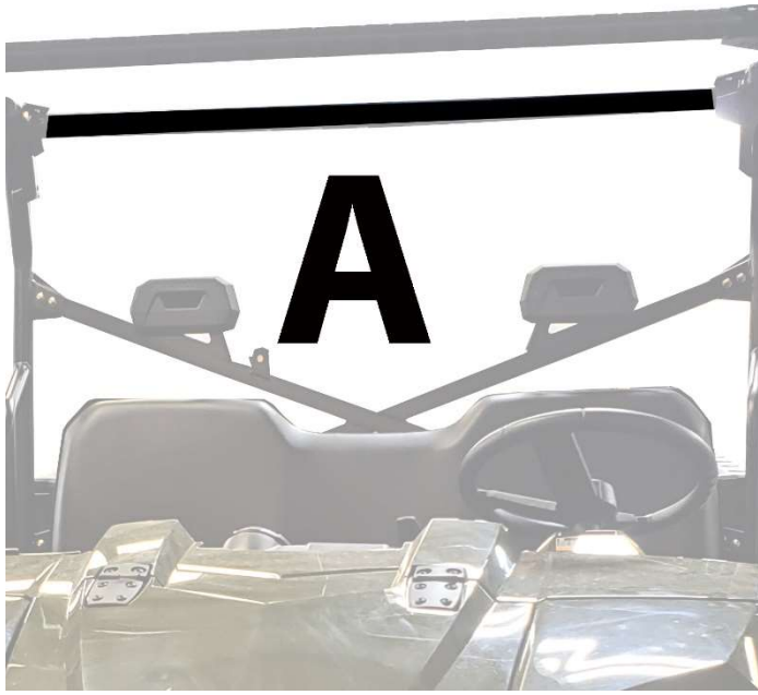
Figure 1: This strip will stretch all the way across the back roll bar. Pull the top of the back panel up and over the top of the roll bar and attach. YOU MAY CHOOSE TO CUT THIS STRIP IN HALF FOR EASIER INSTALLATION.
