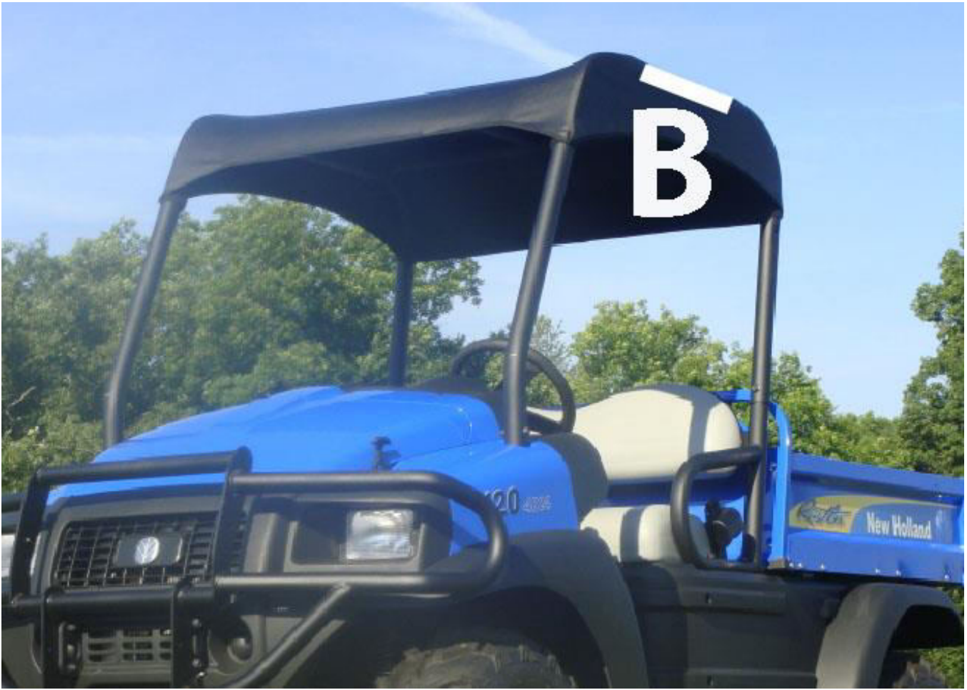
Figure 2: PLACE ADHESIVE VELCRO HORIZONTAL ON THE TOP SIDE ROLL BAR. PULL TAB OVER THE TOP OF THE BAR AND ATTACH TO ADHESIVE STRIPS.
