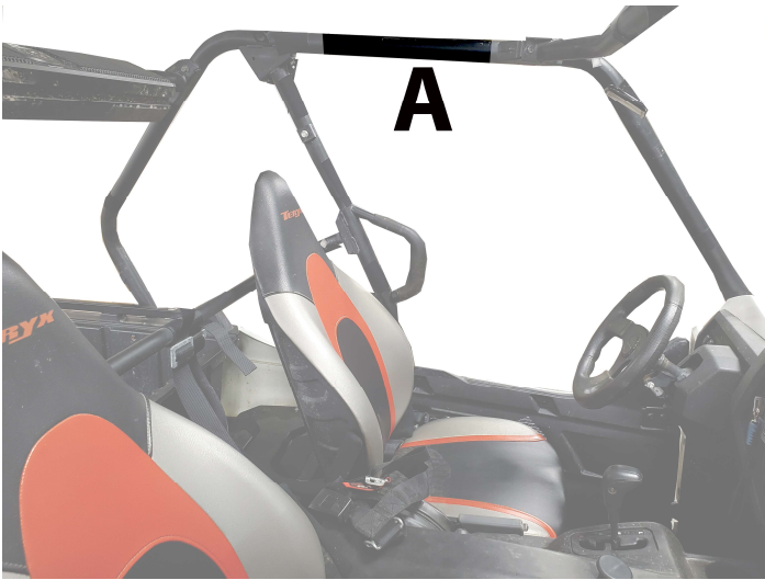
Figure 1: Shows placement of Velcro strips A. The tab on the top of the door kit will pull up and over the roll bar.
