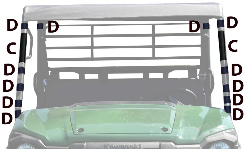
Figure 1: Shows placement of 12" and 6" Velcro strips C and D. The tabs on the front of your doors will wrap around the front of the roll bar and attach to the Velcro strip. Strips D are for the double sided straps that wrap around the roll bar.
