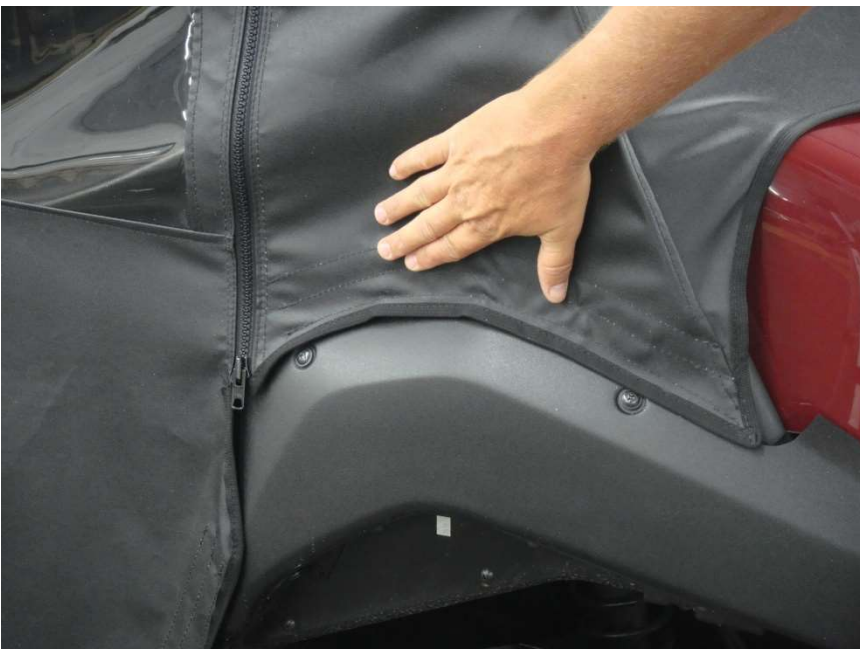
Figure 11.1 - attach Dash Cowl side Velcro Tabs
