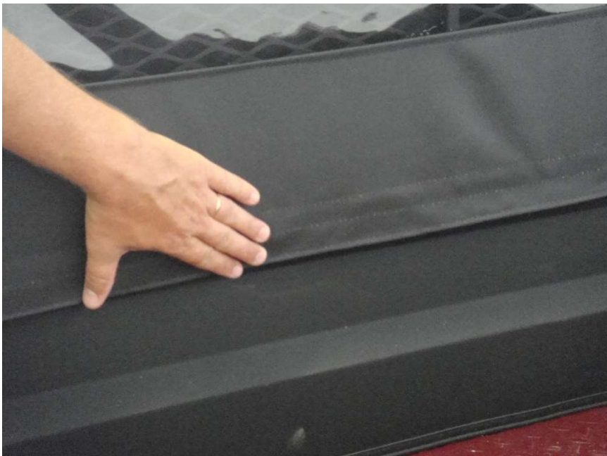
Figure 6.1 - square rear of enclosure to cab and attach rear enclosure Velcro tab to installed 46" Velcro strip
