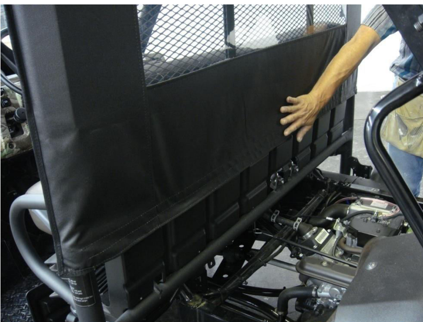
Figure 6.1 - square enclosure to frame and attach 49" rear cab Velcro tab to installed Velcro Strip
