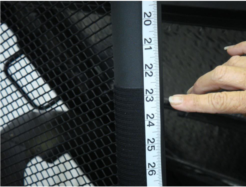
Figure 2.4 - 8" Velcro Strips placed 23" below the top rear cab roll bar cross-member bolted section
