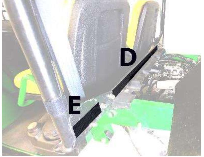
Figure 3: Shows placement of 29" Velcro strip D and 8" Velcro strip E.
