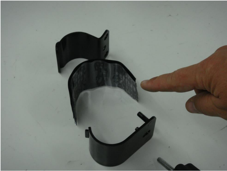
Figure 3.2 - attach sticky Velcro horizontally around the roll bar underneath each clamp bracket before attaching clamps
