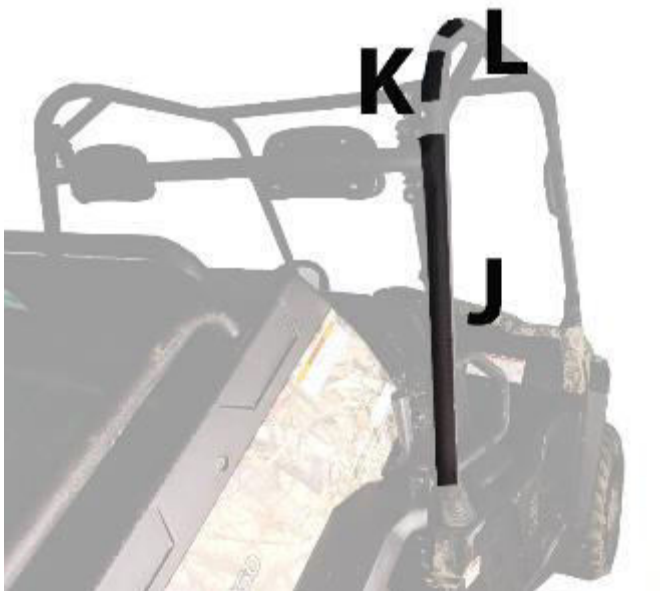
Figure 5: Photo shows placement of Velcro strips J, K AND L. If you ordered a door rear window the rear window will have Velcro sewn on the outside of the panel.
