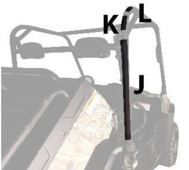
Figure 5: Photo shows placement of Velcro strips J, K AND L. If you ordered a door rear window the rear window will have Velcro sewn on the outside for these strips.
